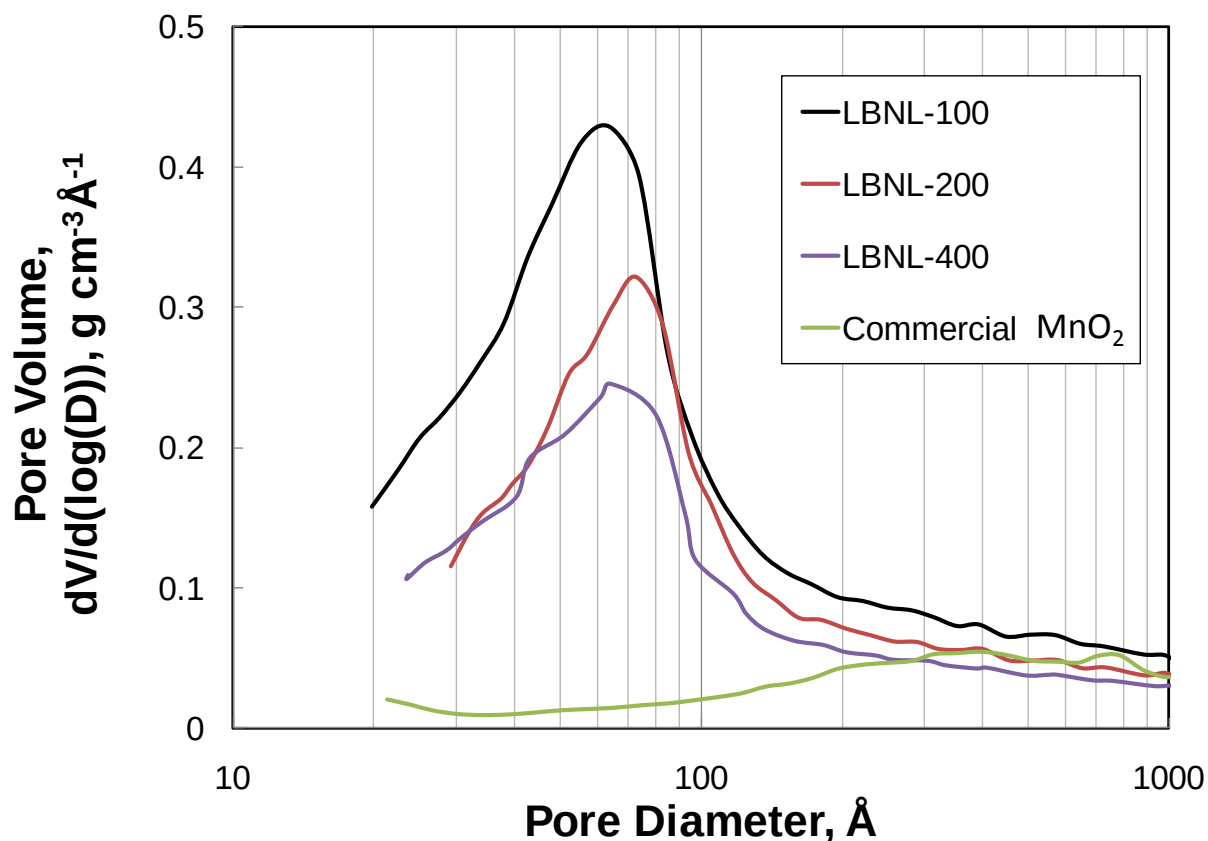
Figure 1. BJH pore size distribution of synthesized samples and commercial MnO 2 .
