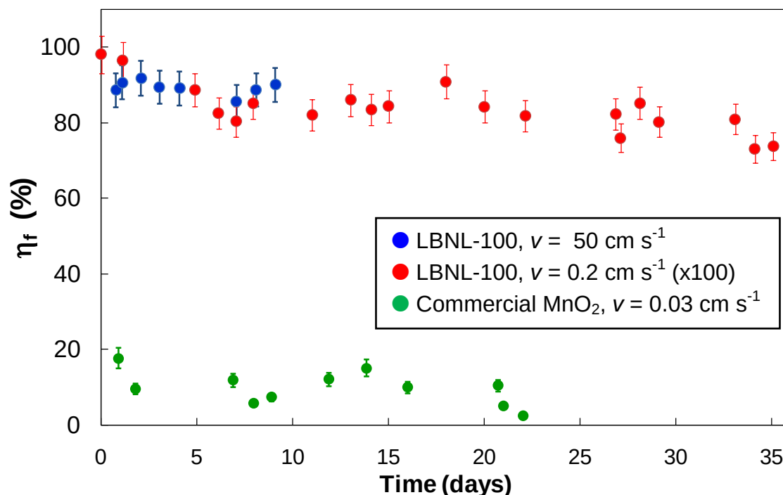
Figure 4. Formaldehyde removal \eta_f vs. time.
